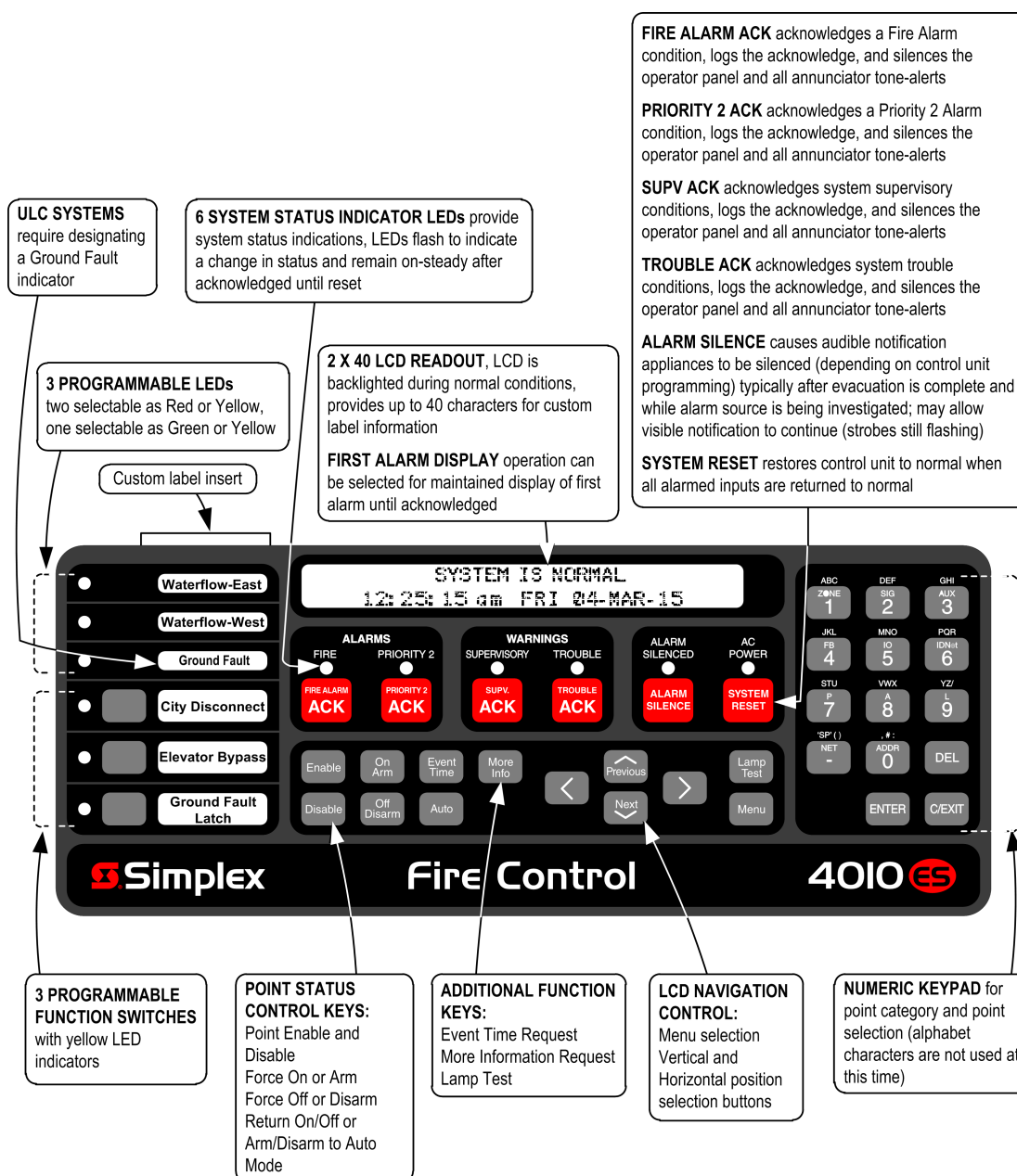
Figure 16: Primary functions of the operator interface
