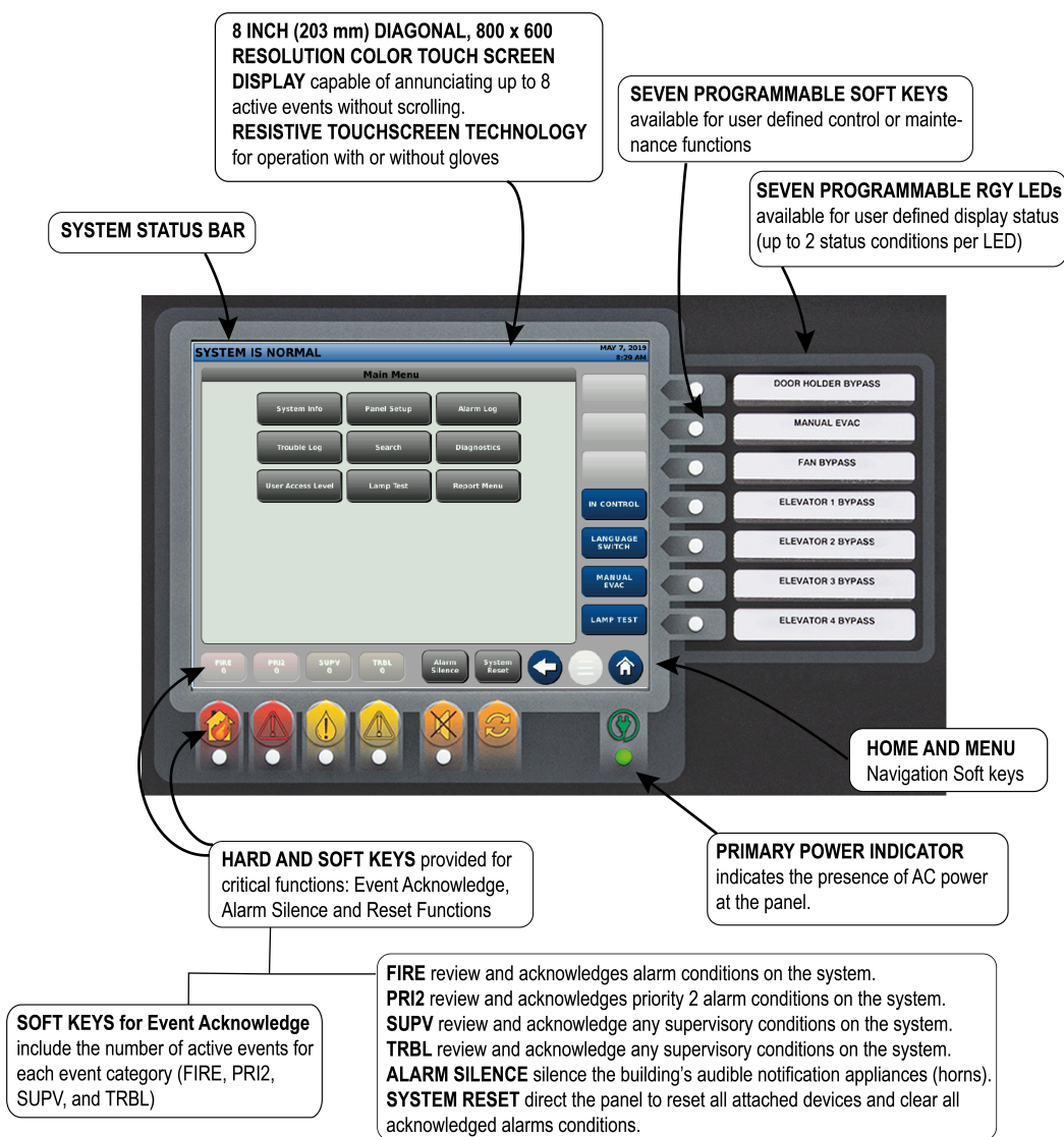
Figure 9: ES Touch screen display operator interface
