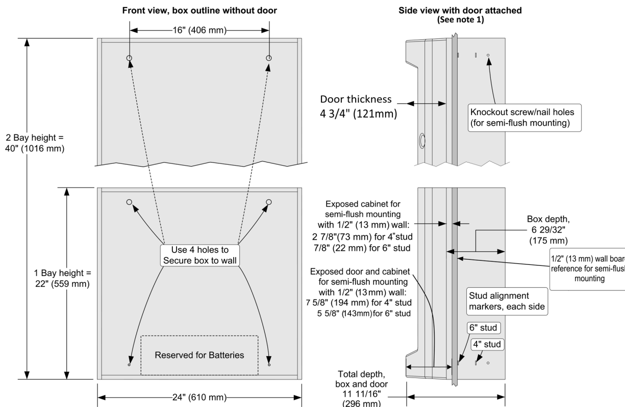
Figure 17: Cabinet dimensions
