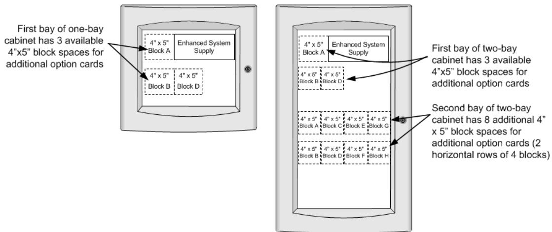
Figure 18: Cabinet one and two bay loading reference
